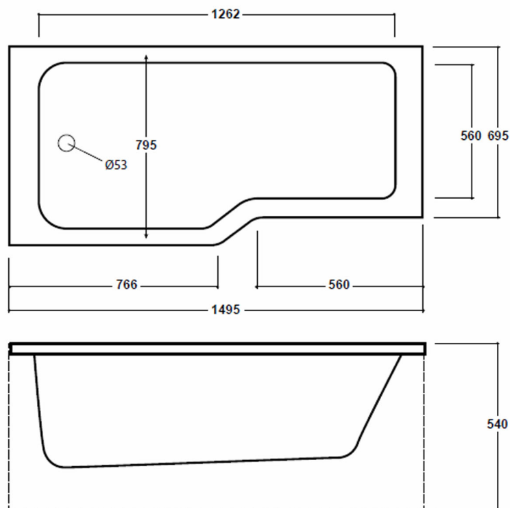
L shaped shower bath 1500mm SY-115LH - left / SY-115RH - right
