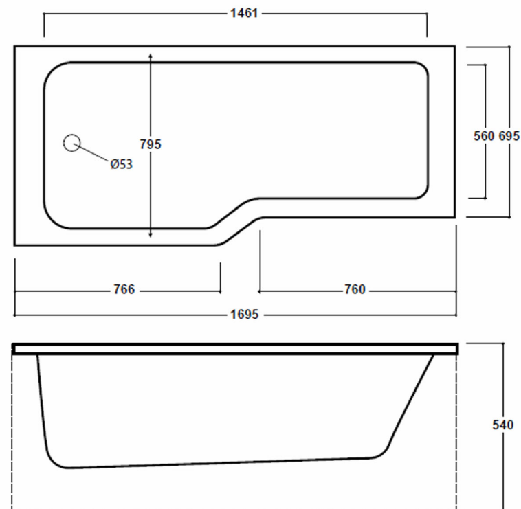
L shaped shower bath 1700mm SY-117LH - left / SY-117RH - right
