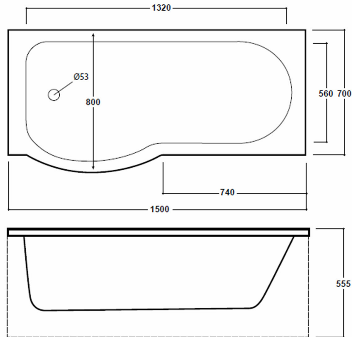
P shaped shower bath 1500mm SY-ZB15LS - left / SY-ZB15RS - right
