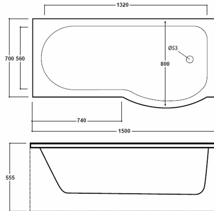
P shaped shower bath 1700mm SY-ZB17LS - left / SY-ZB17RS - right
